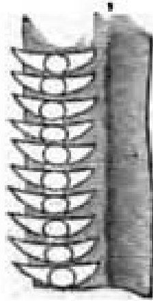
FIG. 11. —Teeth of Nervure of Gryllus domestica (from Landois).
