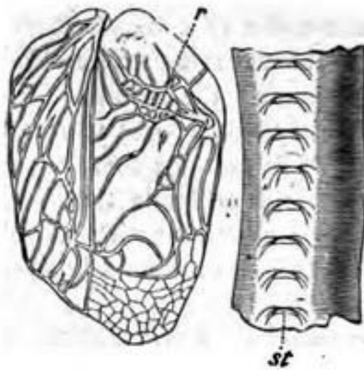
FIG. 10. — Gryllus campestris (from Landols). Right-hand figure, under side of part of the wing-nervure, much magnified, showing the teeth, st . Left-hand figure, upper surface of wing-cover, with the projecting, smooth nervure, r , across which the teeth ( st ) are scraped.
