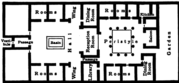
FIG. 29. — TYPICAL SCHEME OF ROMAN HOUSE.
