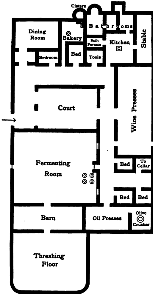
FIG. 45.—PLAN OF HOMESTEAD AT BOSCOREALE.
