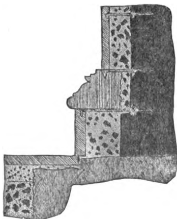
FIG. 28. — BUILDING MATERIALS. (From Middleton.)
